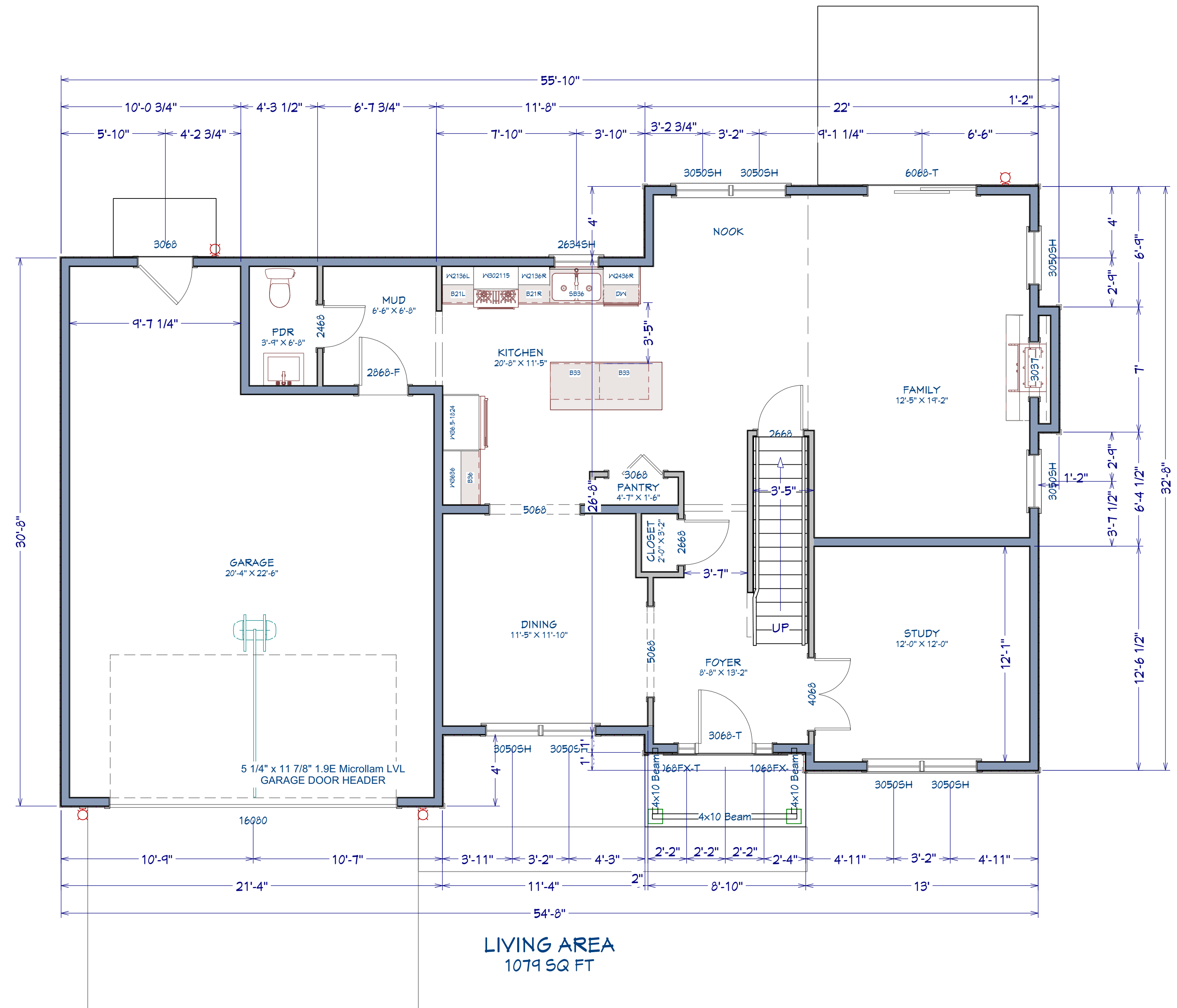
1st Floor
